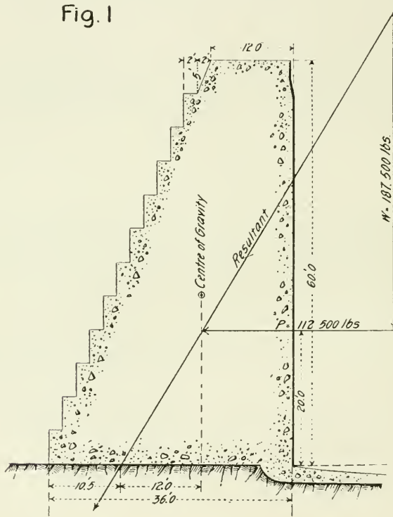
Chamber Wall
