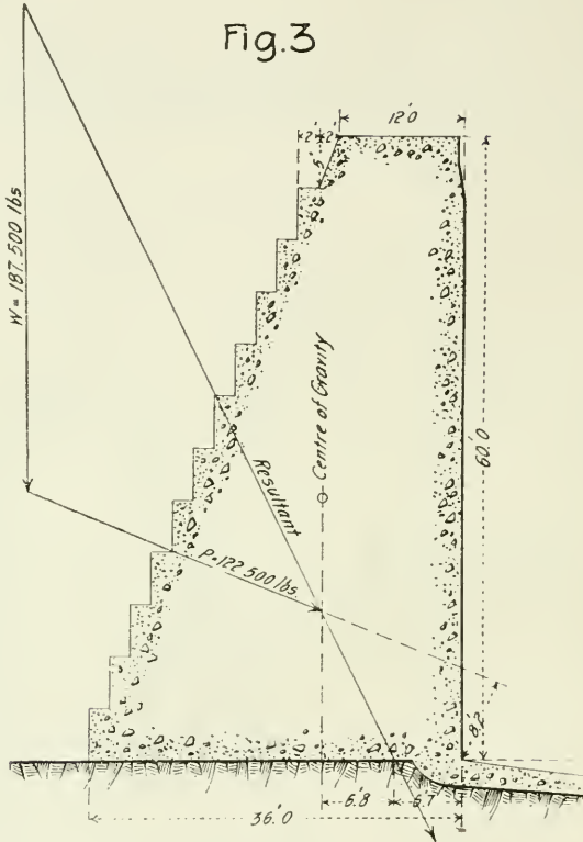
Chamber Wall
