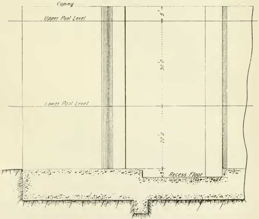
Lower Abutment Wall
