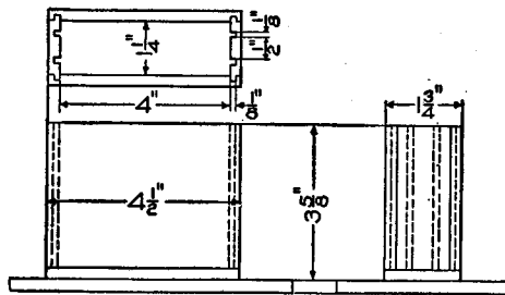
Details of the Developing Box
