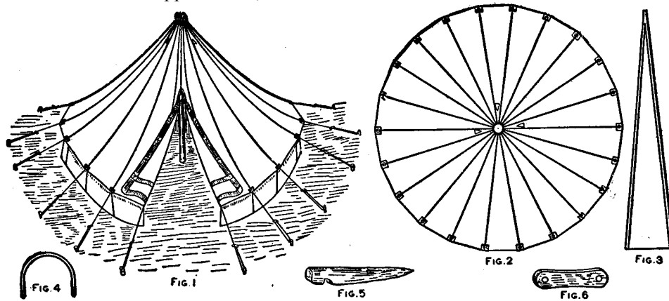
An Inexpensive Home-Made Tent
