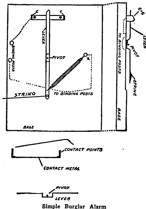
Simple Burglar Alarm
