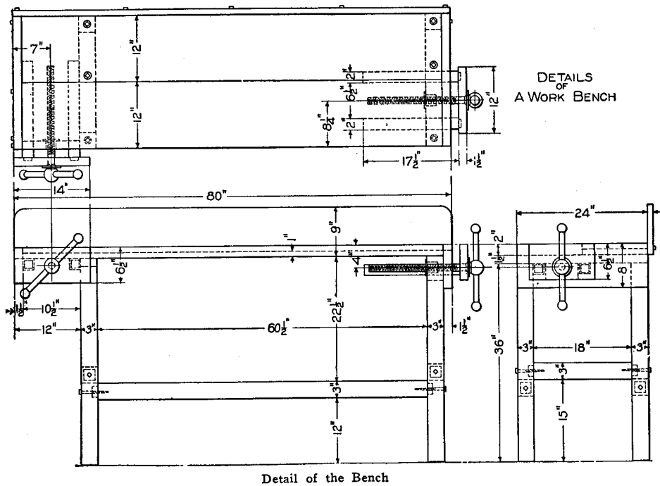
Detail of the Bench
