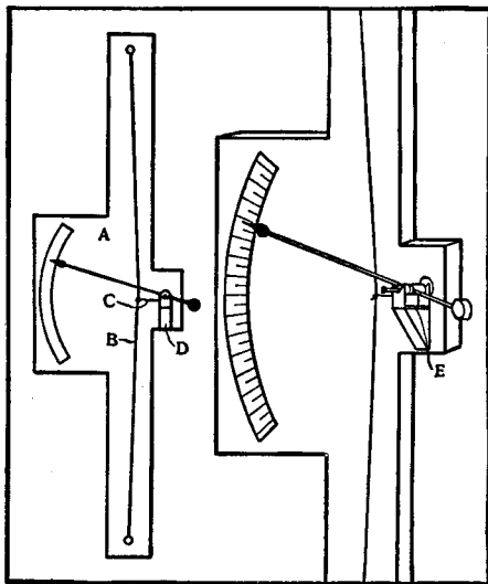
The Hygrometer
