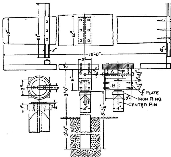
Details of Teeter Board
