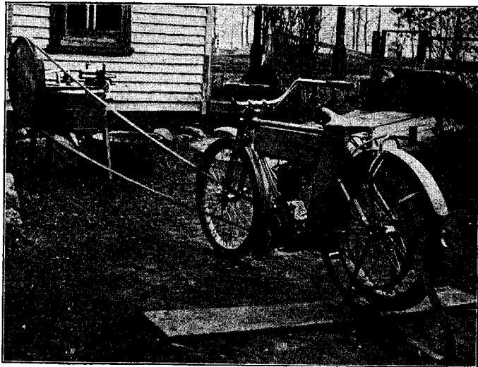
Machine Belted to the Motorcycle
