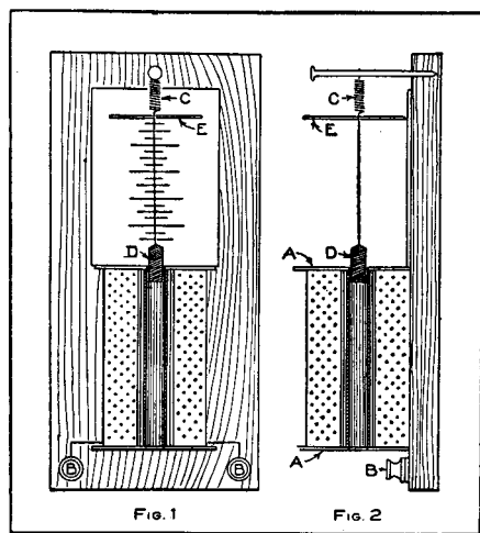
Battery Voltmeter Construction
