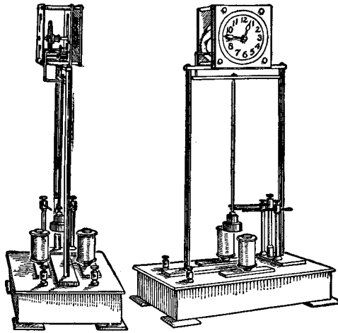
Magnetic Clock
