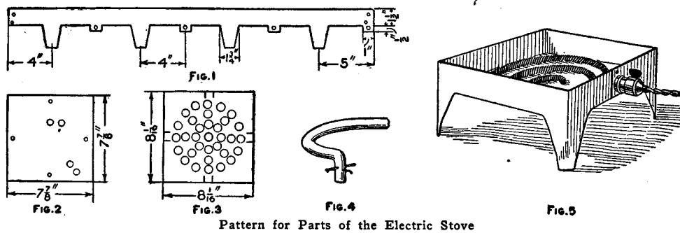
Pattern for Parts of the Electric Stove
