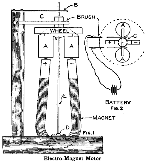
Electro-Magnet Motor
