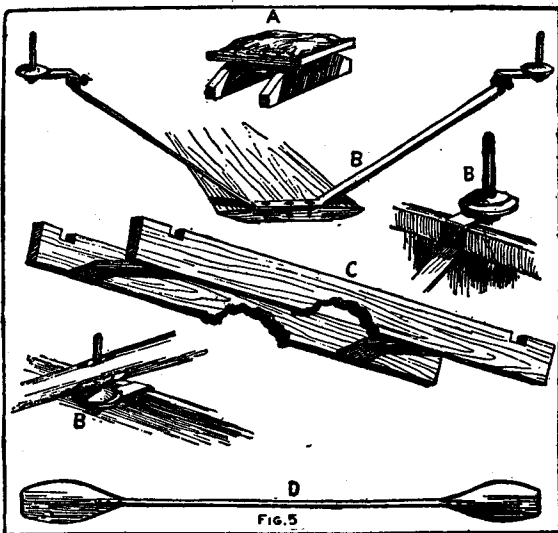
Important Features of Construction
