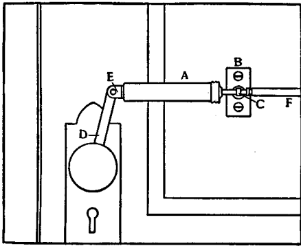
Pneumatic Door-Opener
