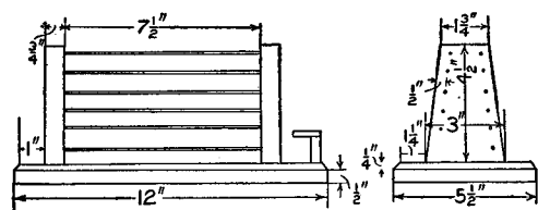
Detail of Toaster
