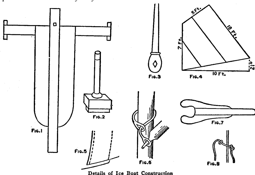
Details of Ice Boat Construction
