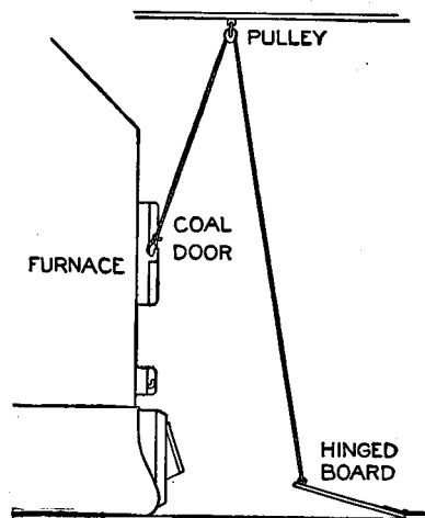
Furnace Door Opener
