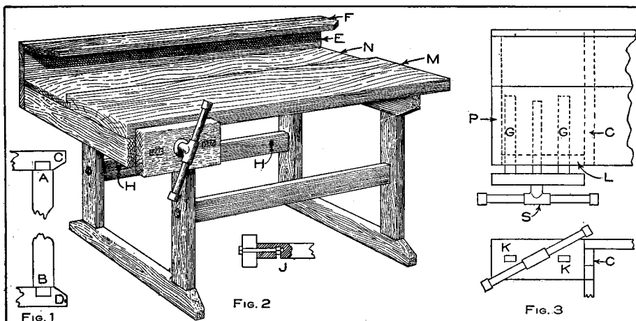
Details of Construction of Homemade Workbench
