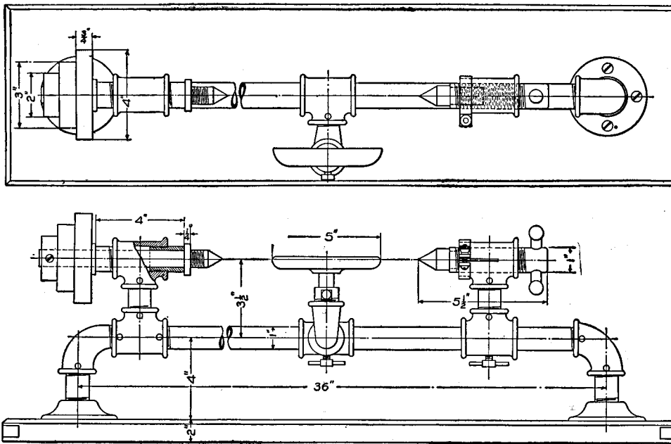
Fig. 1—Details of Lathe
