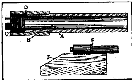
Toy Cannon
