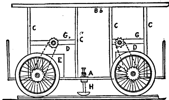
FIG 1 Construction of Car
