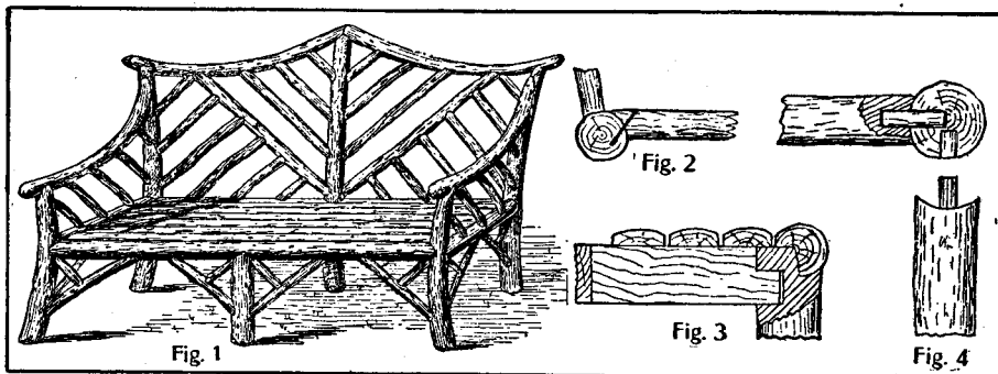
Rustic Seat and Details of Construction Rustic Seat and Details of Construction
