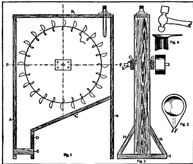
Detail of Homemade Waterwheel
