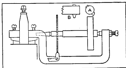
Gear-Cutting Attachment for Lathes
