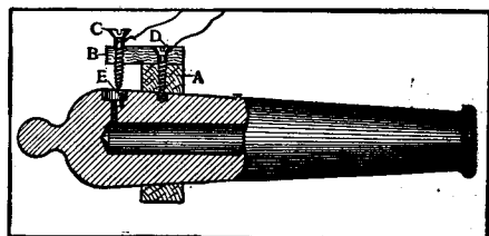
Electrical Attachment for Discharging Toy Cannon
