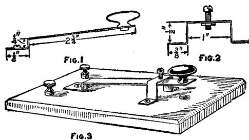
Brass Key on a Wood Base
