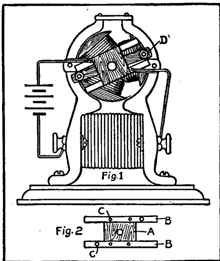
Direct-Connected Reverse
