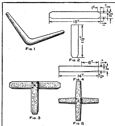
Details of Three Boomerangs
