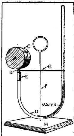
Air Thermometer
