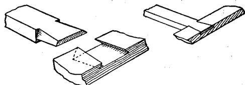
Shape of Tenon and Mortise
