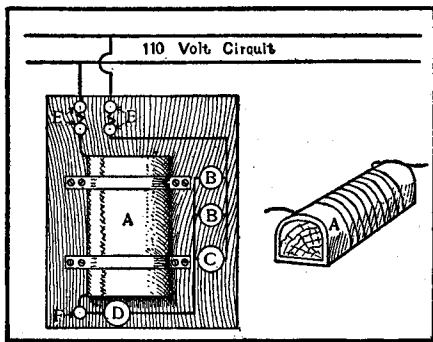
Electric Furnace
