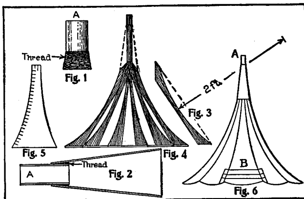
Detail of Phonograph Horn
