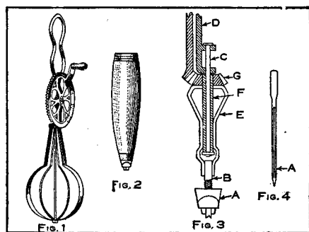
Details of Hand Drill Construction
