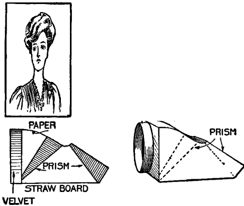
Arrangement of Prisms
