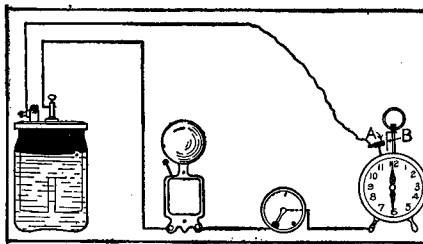
Electric Time Alarm
