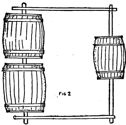
Barrel Float for Bicycle Barrel Float for Bicycle
