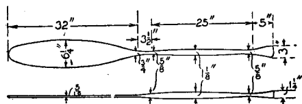
FIG. 13 A Single Paddle
