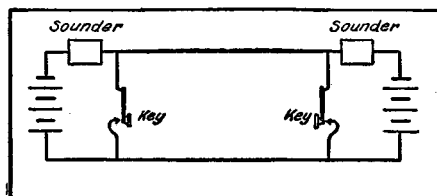
Simple Telegraph Line
