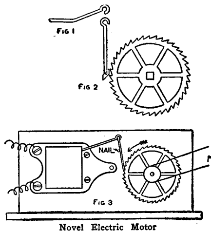
Novel Electric Motor
