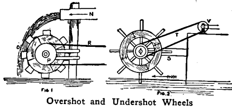
Overshot and Undershot Wheels
