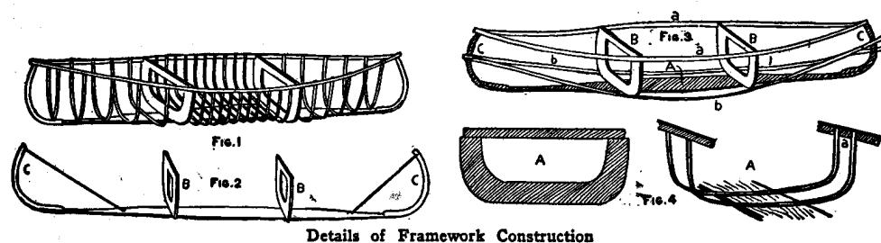
Details of Framework Construction
