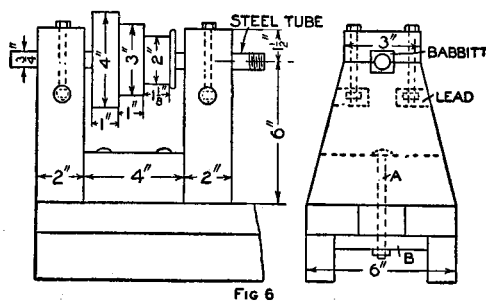
Headstock Details
