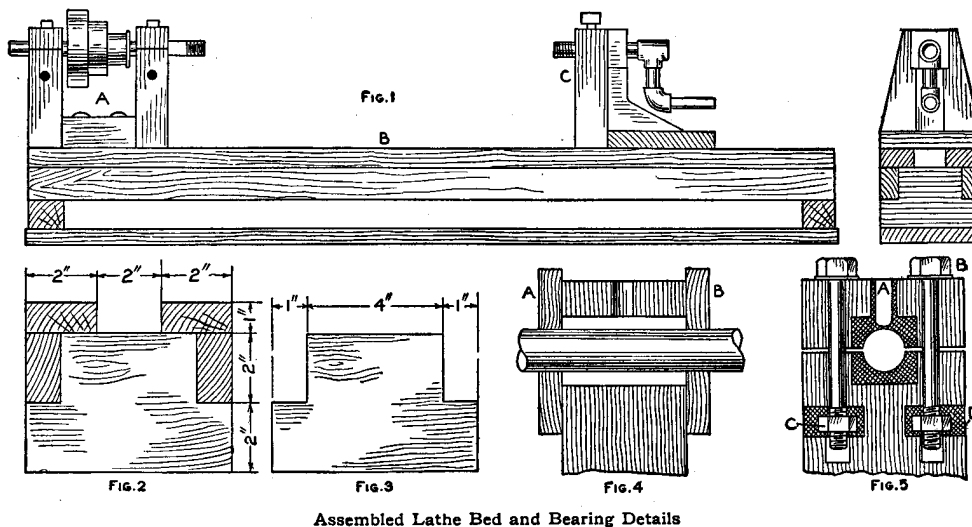
Assembled Lathe Bed and Bearing Details
