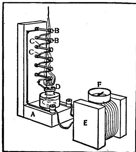
Thermo Battery
