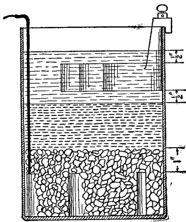
Setting Up a Gravity Battery Setting Up a Gravity Battery
