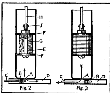
Valve Motion and Construction of Piston
