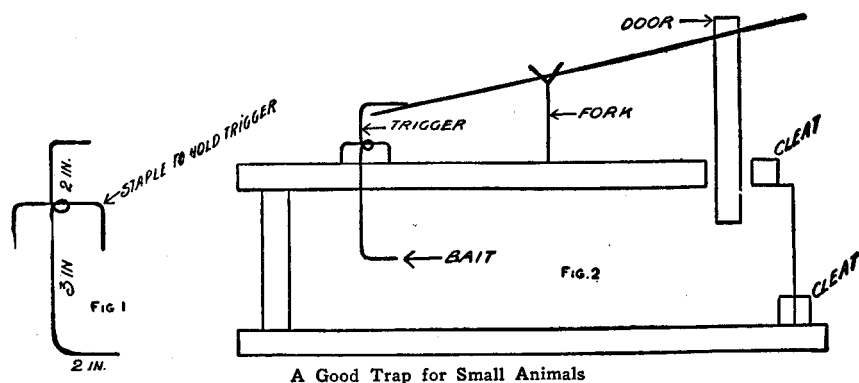
A Good Trap for Small Animals
