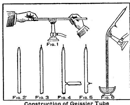
Construction of Geissler Tube
