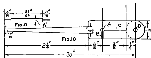
Shaft for Needle and Needle
