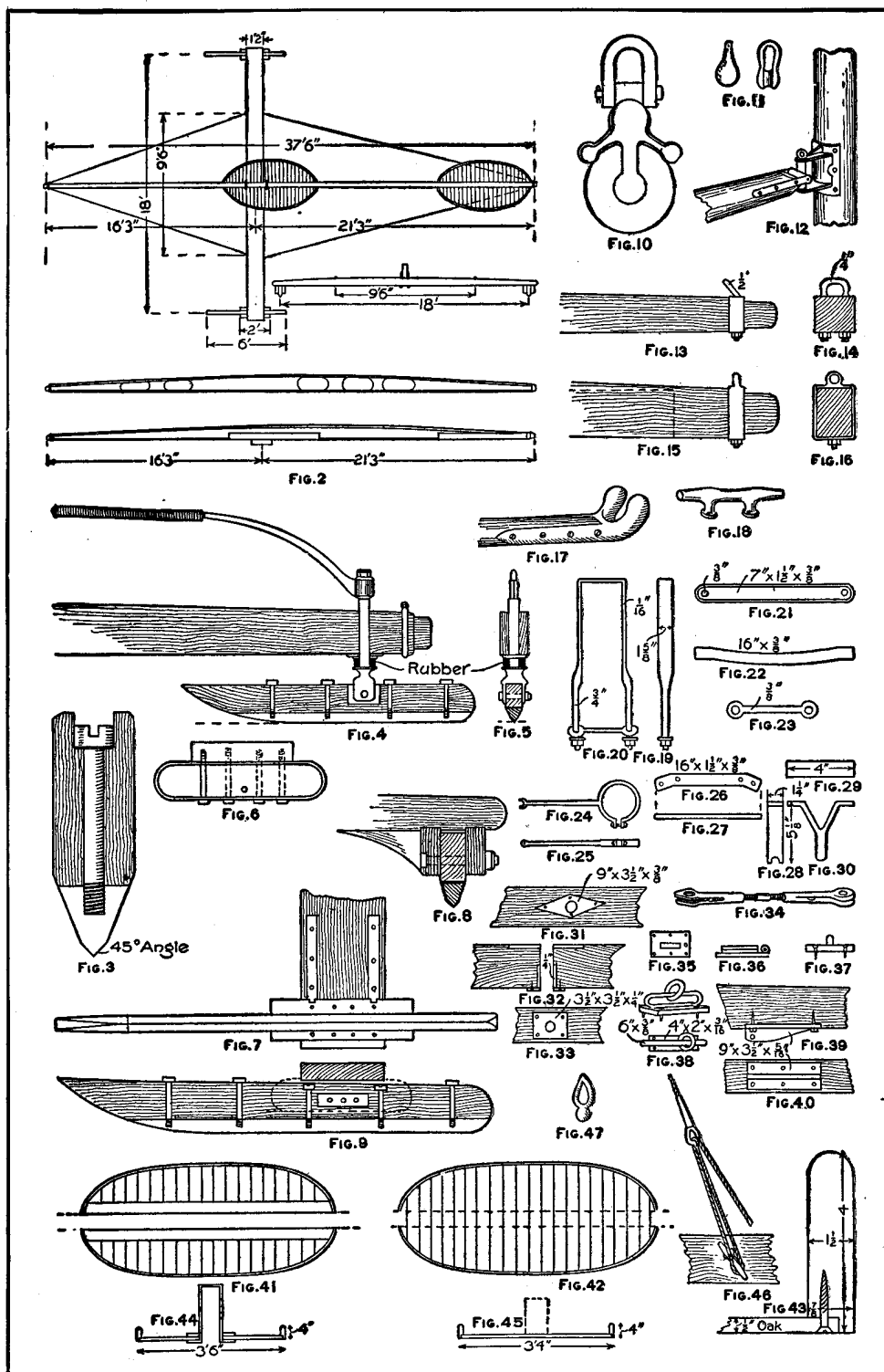
Details of the Ice-Yacht Parts
