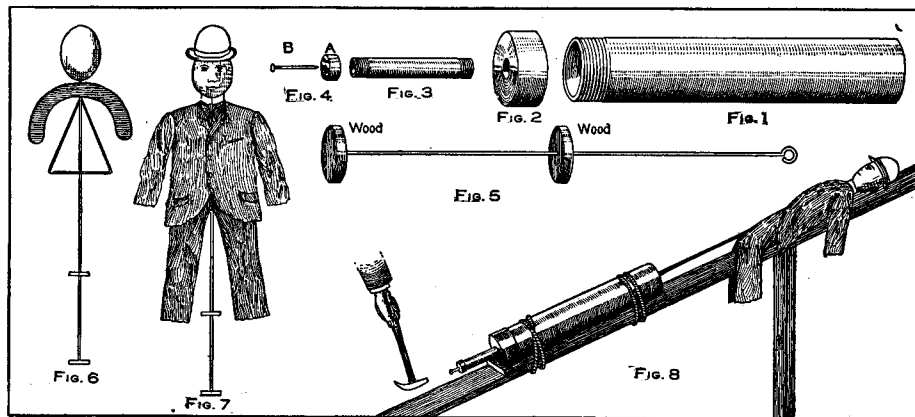
Homemade Cannon Which will Hurl a Life-Size Dummy 100 Ft. through the Air
