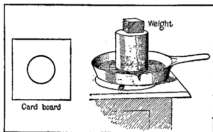
Experimental Apparatus
