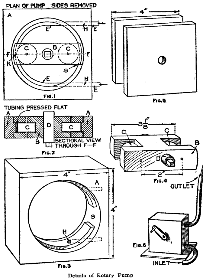
Details of Rotary Pump
