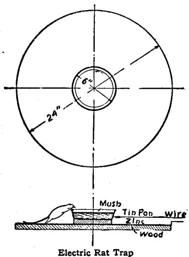
Electric Rat Trap
