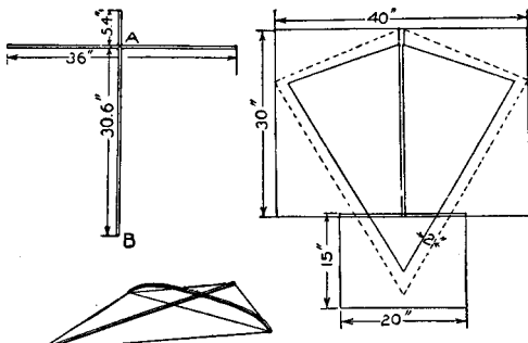
Plan and Dimensions for Kite
