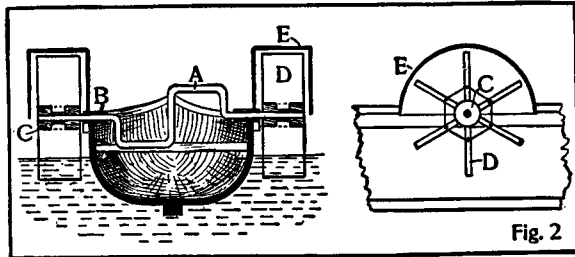
Detail of Paddle Boat
