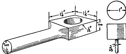
Parts of the Top
