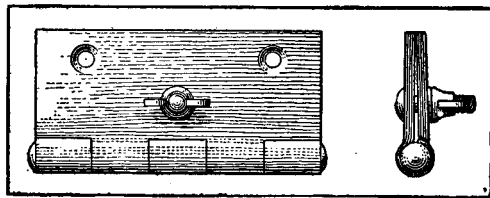
Hand Vise Made from a Hinge
