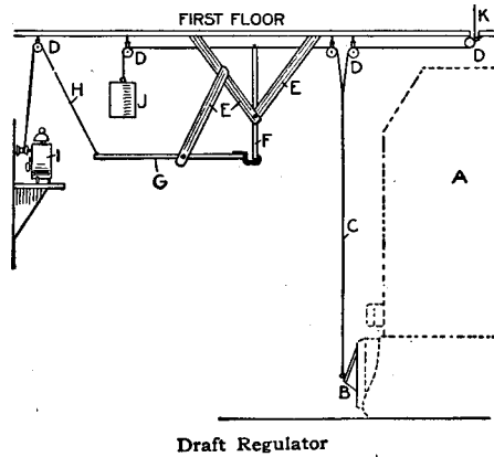
Draft Regulator
