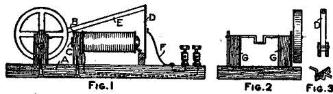
Shaft Turned by Magnetism
