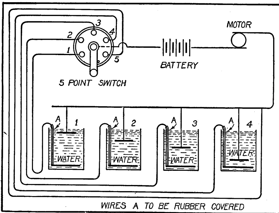
Wiring Plan for Water Rheostat
