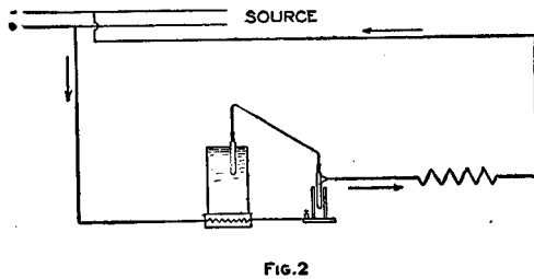
Wiring Diagram Showing How the Connections to a Source of Current Supply are Made
