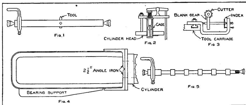
Steps in Making the Home-Made Gasoline Engine
