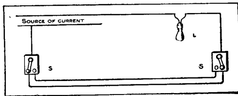
The Wiring Diagram
