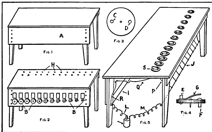
How the Electric Piano is Constructed
