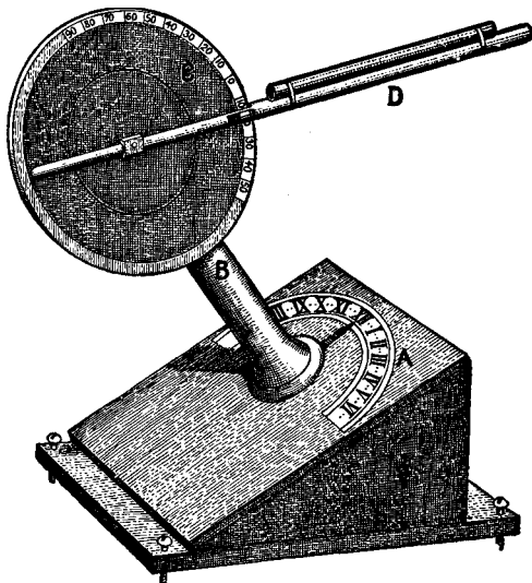
Home-Made Equatorial
