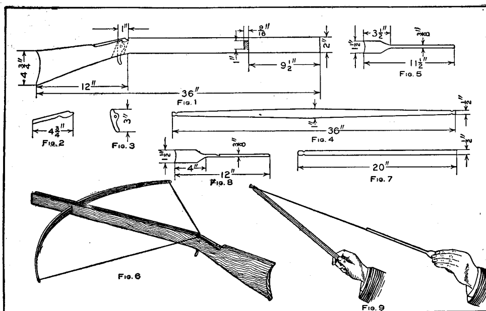
Details of the Bow-Gun and Arrow Sling
