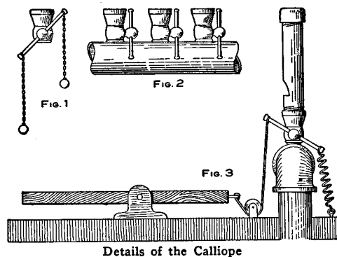
Details of the Calliope
