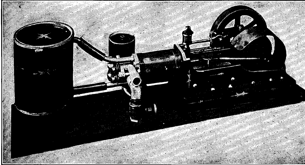
Complete Homemade Gasoline Engine
