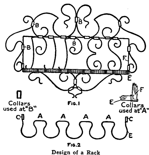
Design of a Rack
