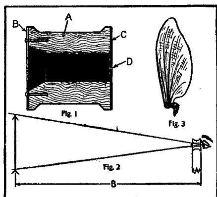
Detail of Lensless Microscope
