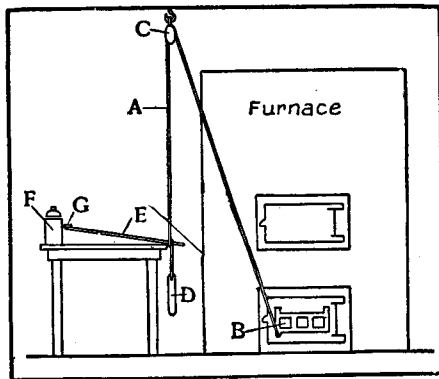
Automatic Time Draft-Opener
