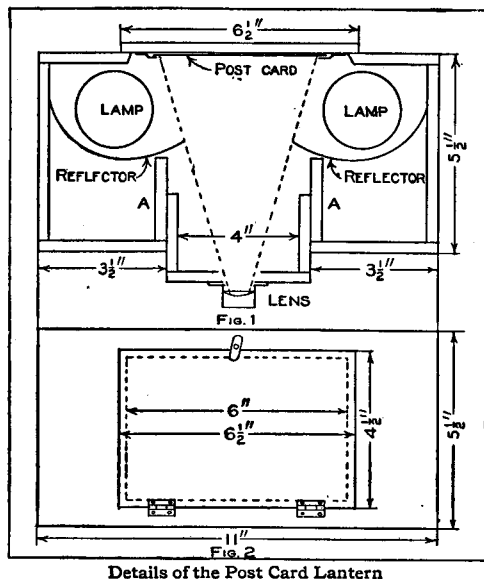
Details of the Post Card Lantern
