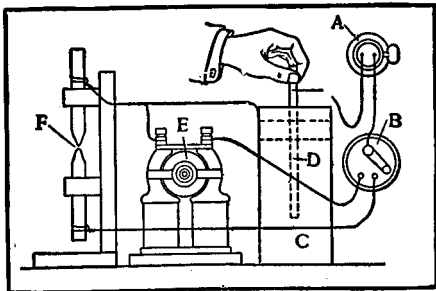
Arc-Light Motor and Water Rheostat
