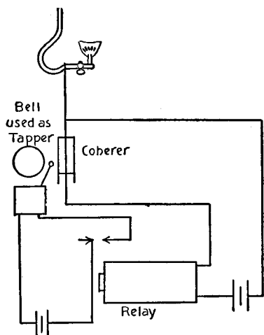
Touch the Gas Jet and Ring the Bell Touch the Gas Jet and Ring the Bell
