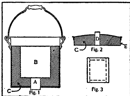
Homemade Pottery Kiln
