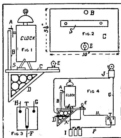
Details of Alarm Construction
