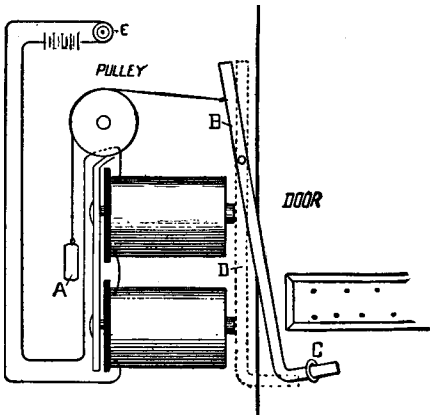
Automatic Electric Lock for Doors
