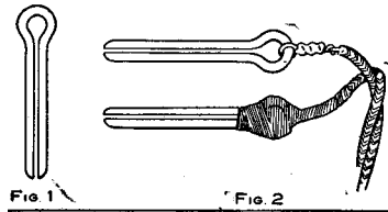
Cotter Pin Wire Terminals
