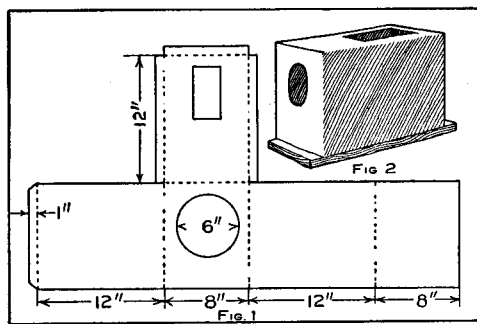
Lantern House
