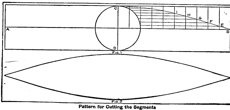
Pattern for Cutting the Segments
