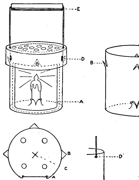
Lantern Made of Old Cans
