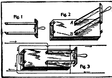
Simple Current-Reversing Switch
