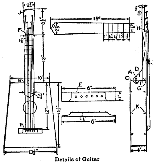
Details of Guitar
