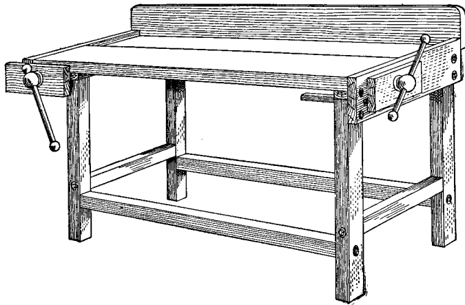
Workbench Complete
