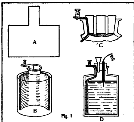
Details of Interrupter
