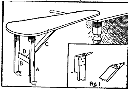
Ironing-Board Stand
