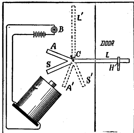
Lock Operated by a Magnet
