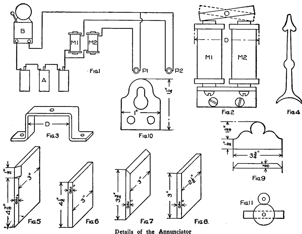
Details of the Annunciator
