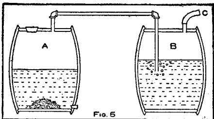
The Hydrogen Generator
