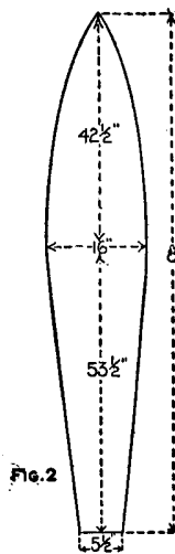
Pattern and Parts to Make Balloon
