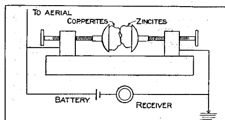
Details of the Receiving Instrument
