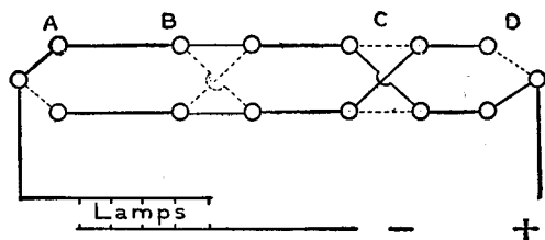
Wiring Diagram
