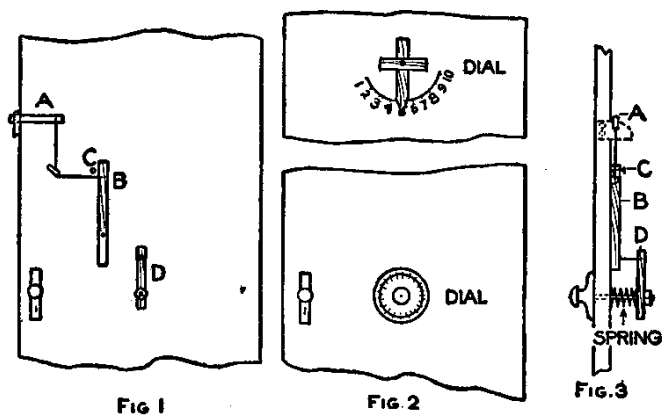
The Lock Parts
