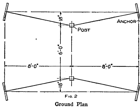
Ground Plan
