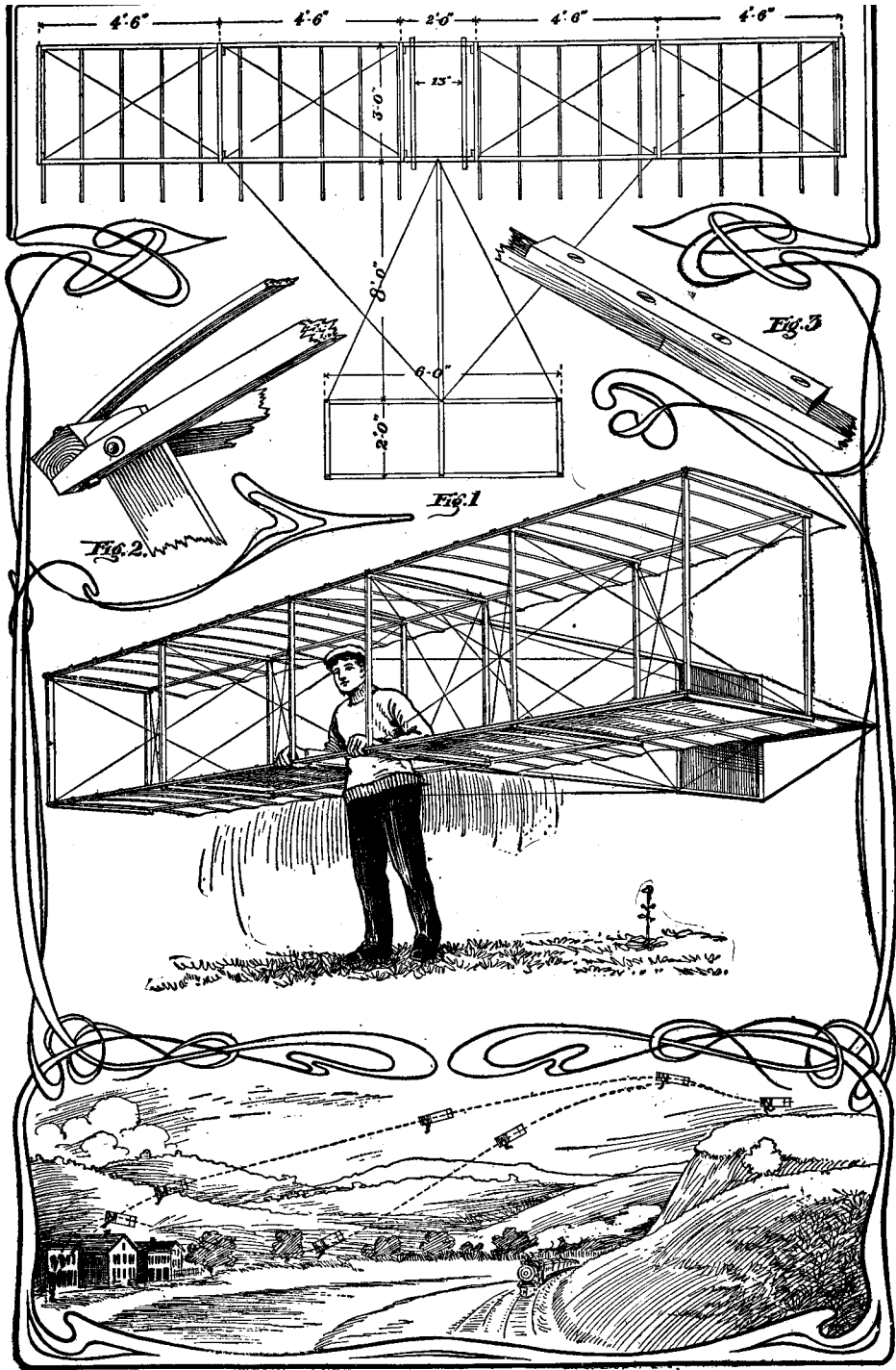
How to Make a Glider (See page 171)
