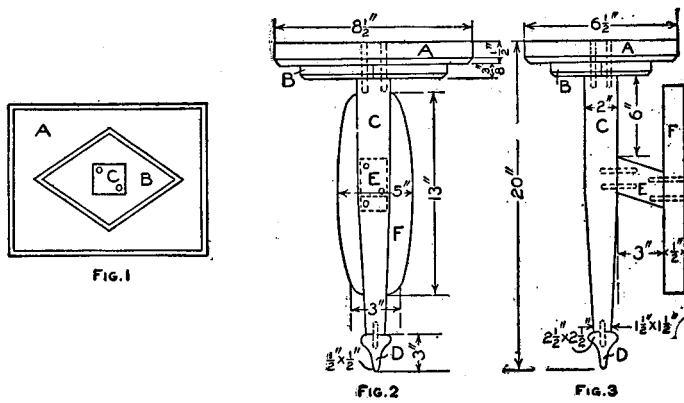
Details of the Wall Bracket
