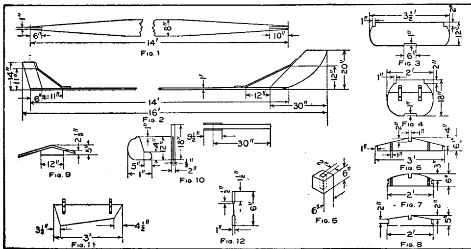
Details of a Home-Made Sailing Canoe
