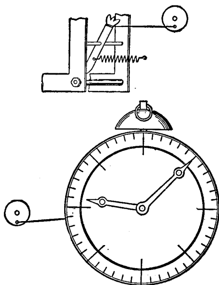
Revolution Recorder Revolution Recorder
