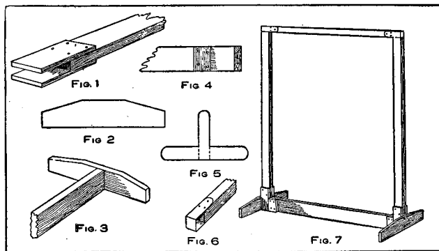
Details of Background Frame
