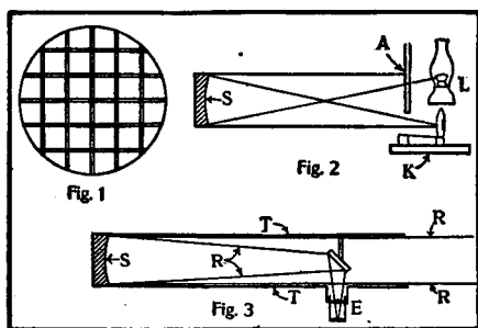
Detail of Telescope Construction
