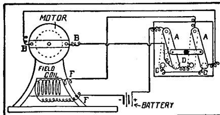
Reverse for a Small Motor
