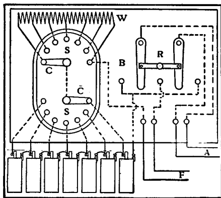
Motor Reverse and Controller
