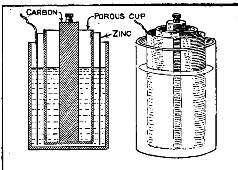
Cross Section and Completed Cell
