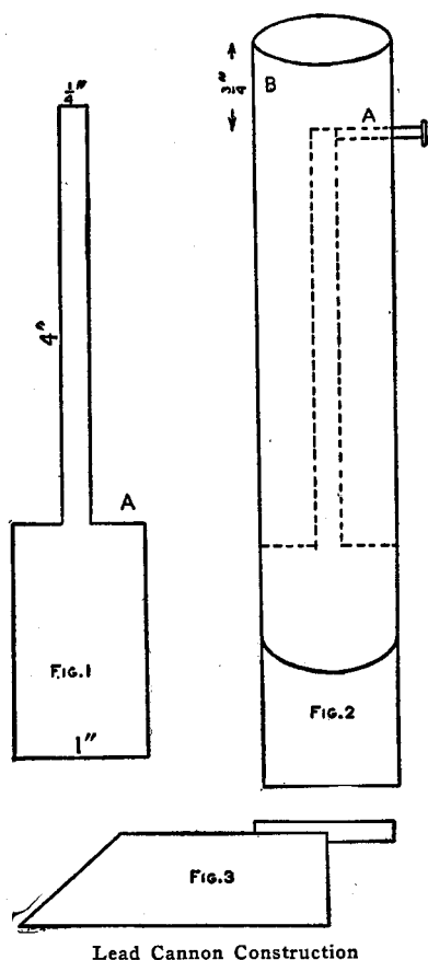
Lead Cannon Construction
