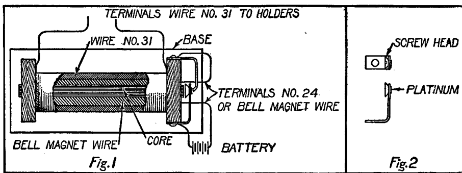
Medical Induction Coil
