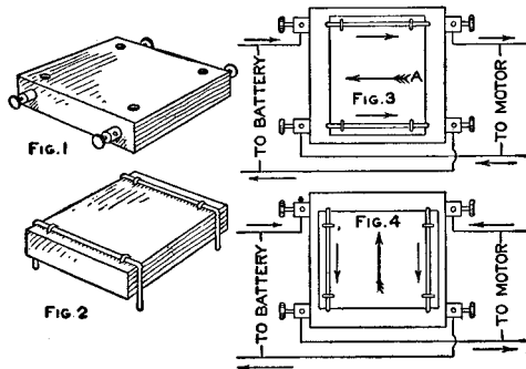
Details of Reverser
