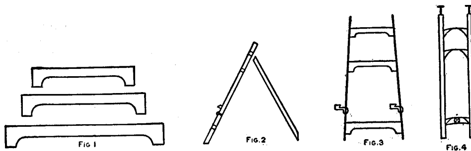
Details of Easel Construction
