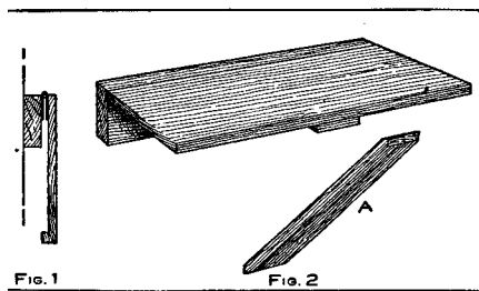
Turn-Down Shelf
