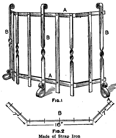
FIG.2 Made of Strap Iron
