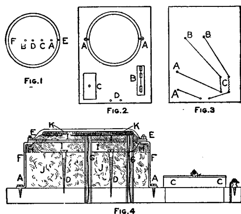
Fig. 4 Details of Electric Stove
