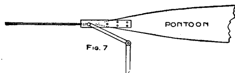
Crosspiece and Rudder Details
