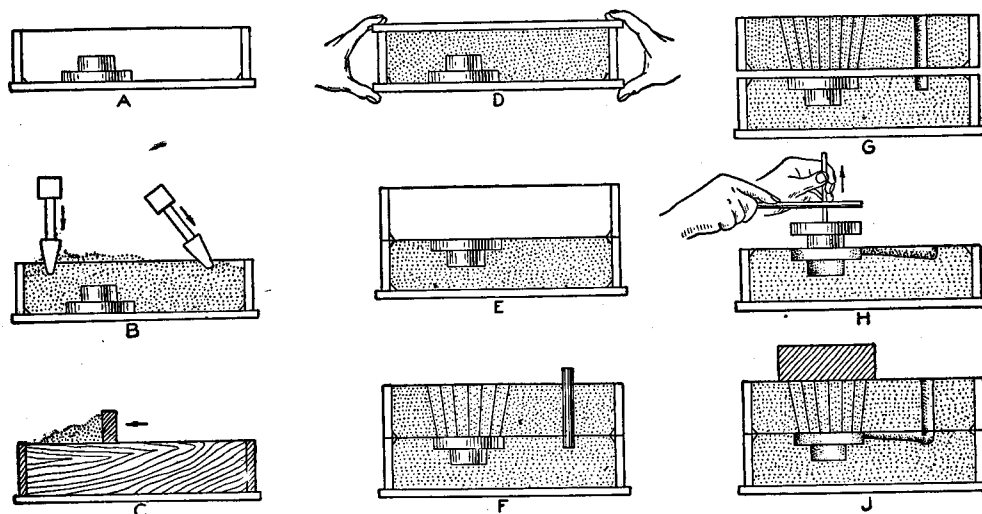
Fig. 3—Making a Mold
