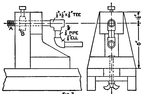
FIG. 7 Details of Tailstock
