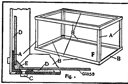
Detail of Aquarium Frame
