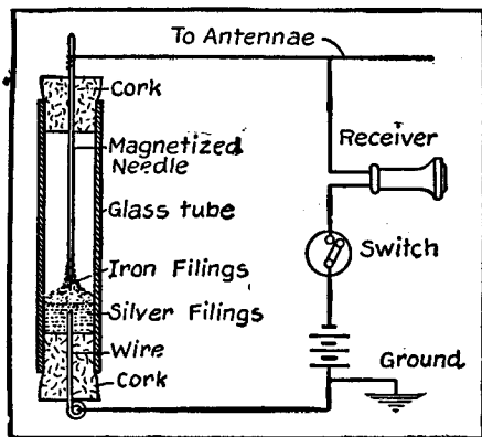
Detail of Coherer
