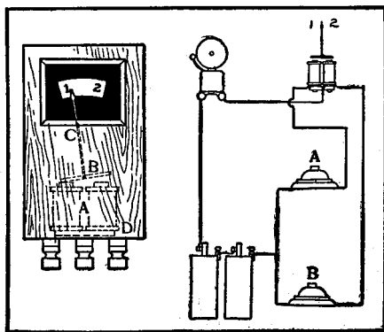
Annunciator and Wiring Diagram
