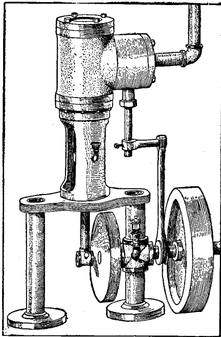
The Engine Is About 20 Inches High
