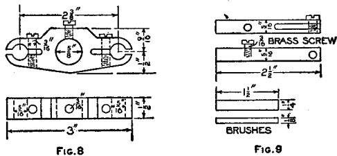
FIG. 8 The Insulated Brush Holder and Its Studs for Holding the Brushes on the Commutator
