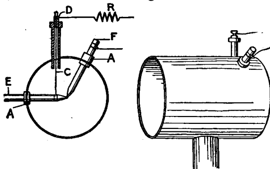
Arc in a Large Tin Can
