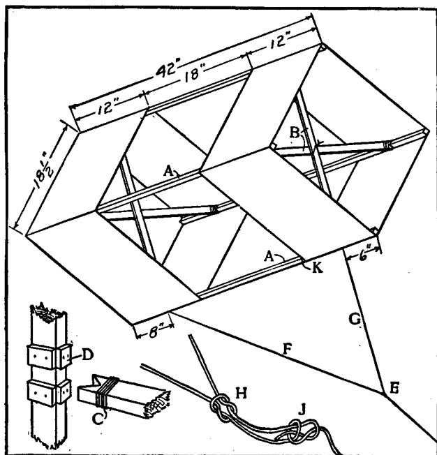
Detail of Box Kite
