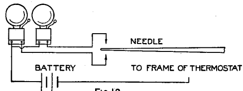
Wiring Diagram for One and Two Bells
