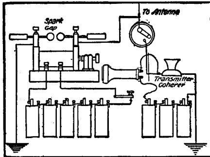
Wiring Diagram for Wireless Telegraph
