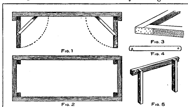
Details of Canvas Cot Construction
