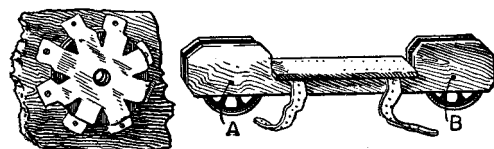
Fig. 1 Fig. 2 Rubber Tired Roller Skate Rubber Tired Roller Skate
