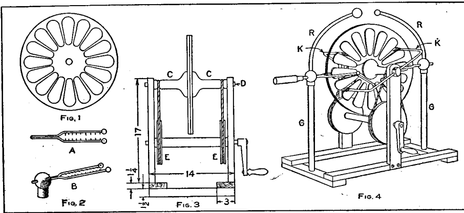
Details of a Homemade Static Machine
