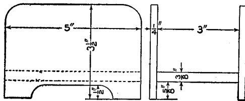
Details of the Rack
