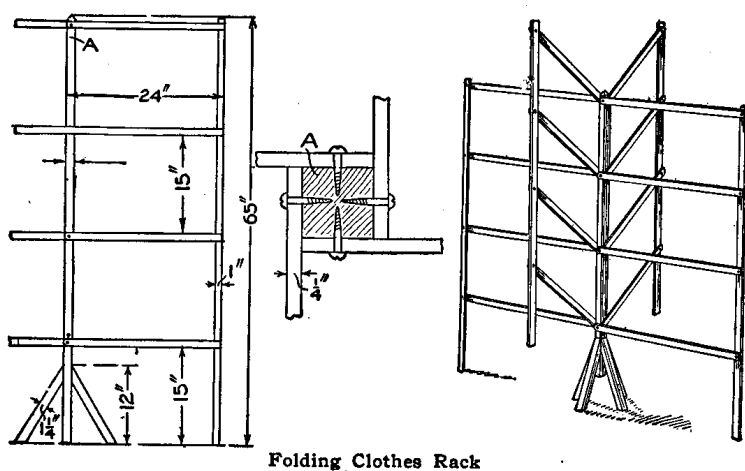
Folding Clothes Rack
