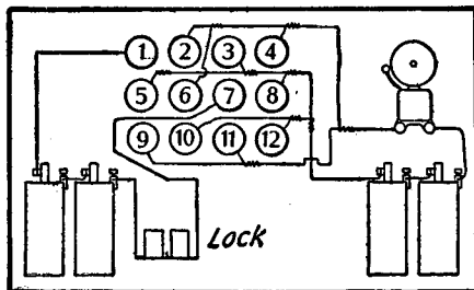
Wiring Diagram
