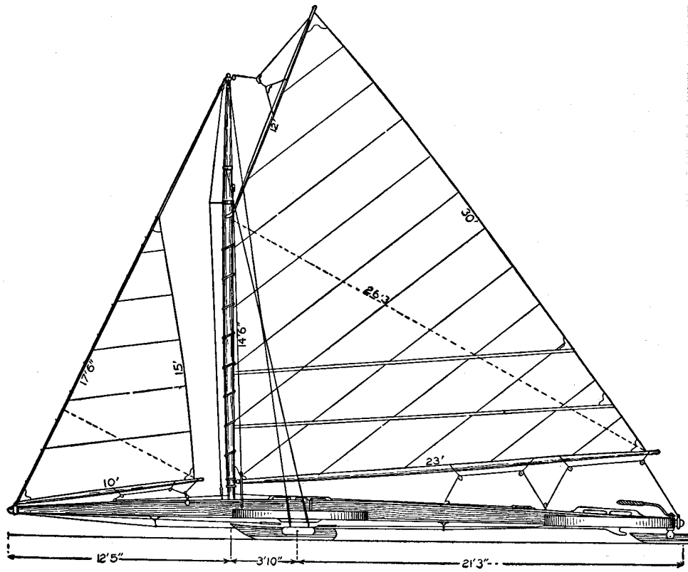
Fig. 1 Ice-Yacht Complete
