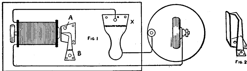
Home-Made Telegraph Instrument
