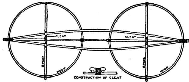
Frame for Skater's Sails
