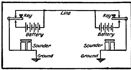
Diagram of One-Wire Line
