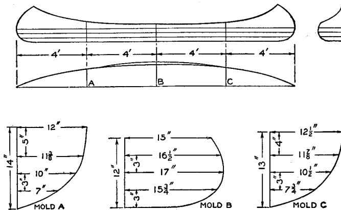
FIG. 1 Canoe and Molds Details
