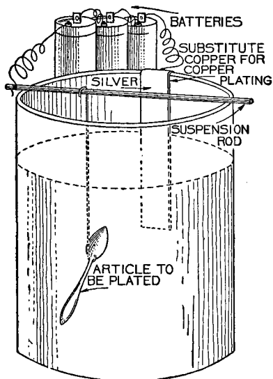
Electroplating Apparatus
