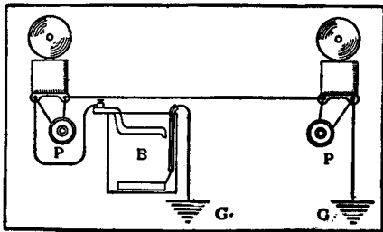
Wiring Diagram
