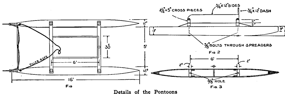
Details of the pontoons
