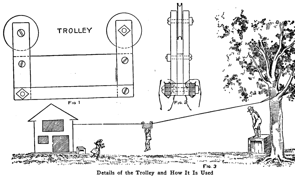
Details of the Trolley and How It Is Used
