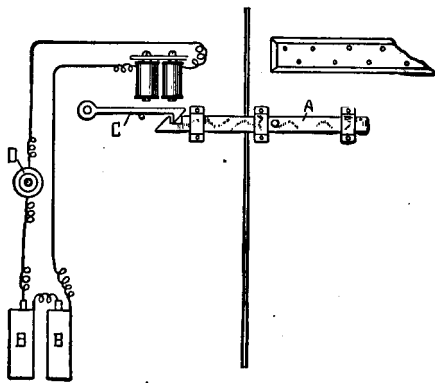
Simple Electric Lock
