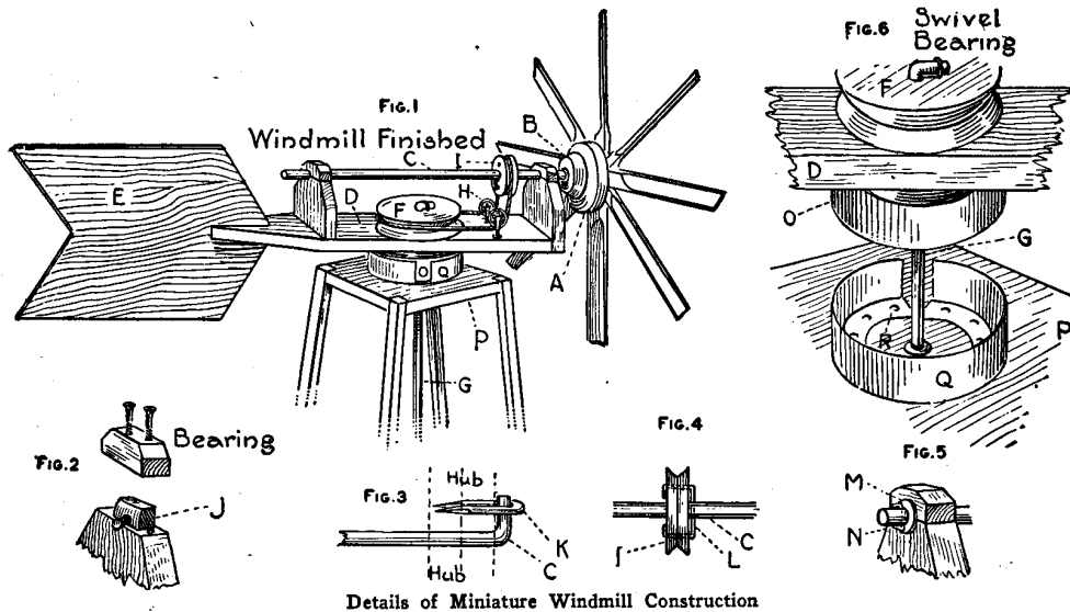
Details of Miniature Windmill Construction
