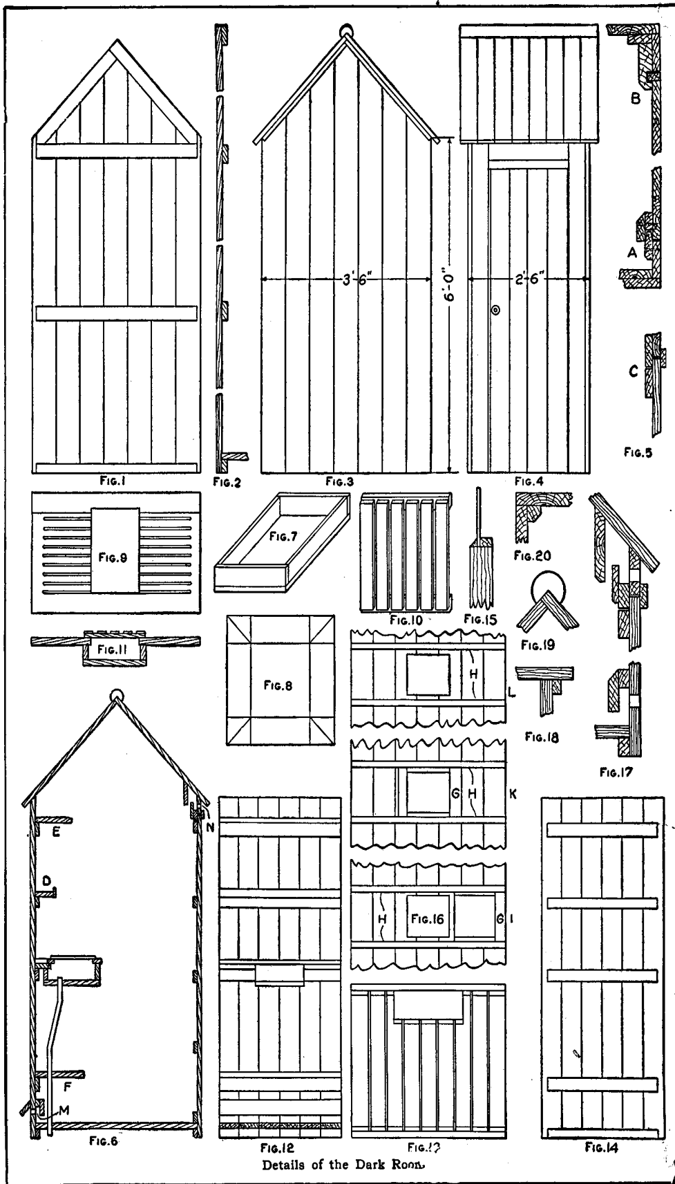
Details of the Dark Room
