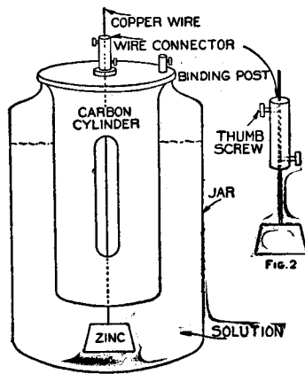
Fig. 1 Details of Homemade Battery
