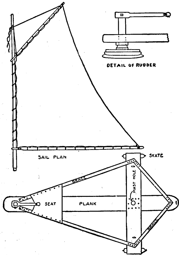
Plan of Ice Boat, Sail and Rudder
