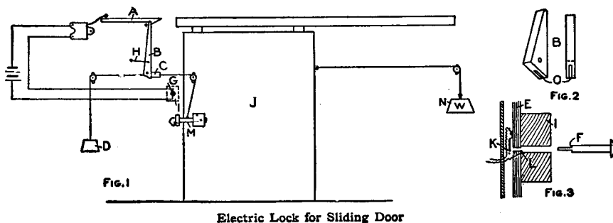
Electric Lock for Sliding Door
