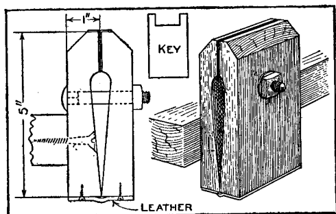
Details of a Home-Made Bench Vice
