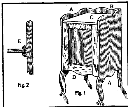
How to Make a Music Cabinet
