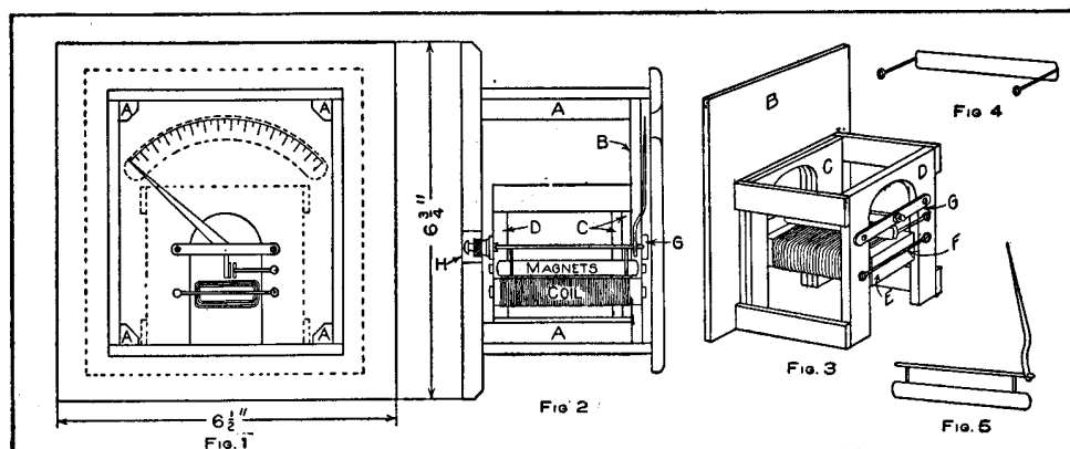
Details of an Ammeter
