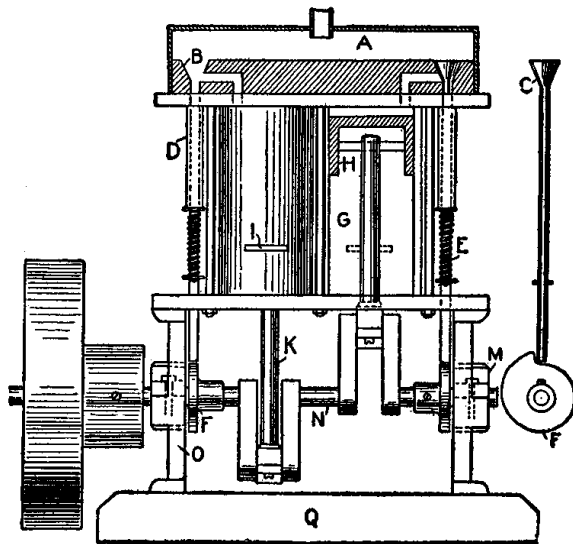
Engine Details
