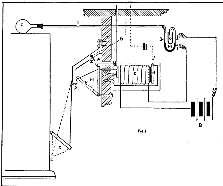
Details of Furnace Regulator Construction
