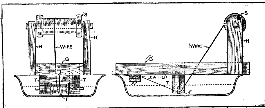
Home-Made Apparatus for Paraffining Wire
