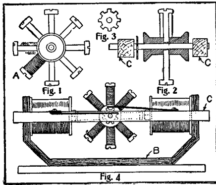
Details of Small Electric Motor
