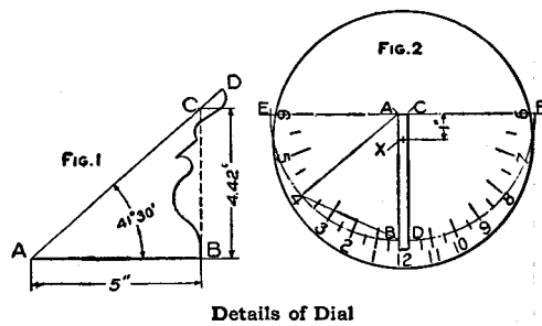
Details of Dial
